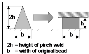
Figure 1: Recommended Bead Configuration
